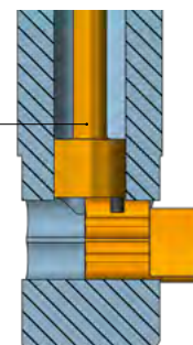
Blade housing with extended blade. The rotary motion of the pinion causes the blade control to extend or retract the blade.
